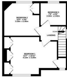
1ST FLOOR 354 sq ft. (32.9 sq.m.) approx.
