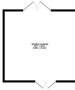
OUTBUILDING 413 sq ft. (38.4 sq.m.) approx.
